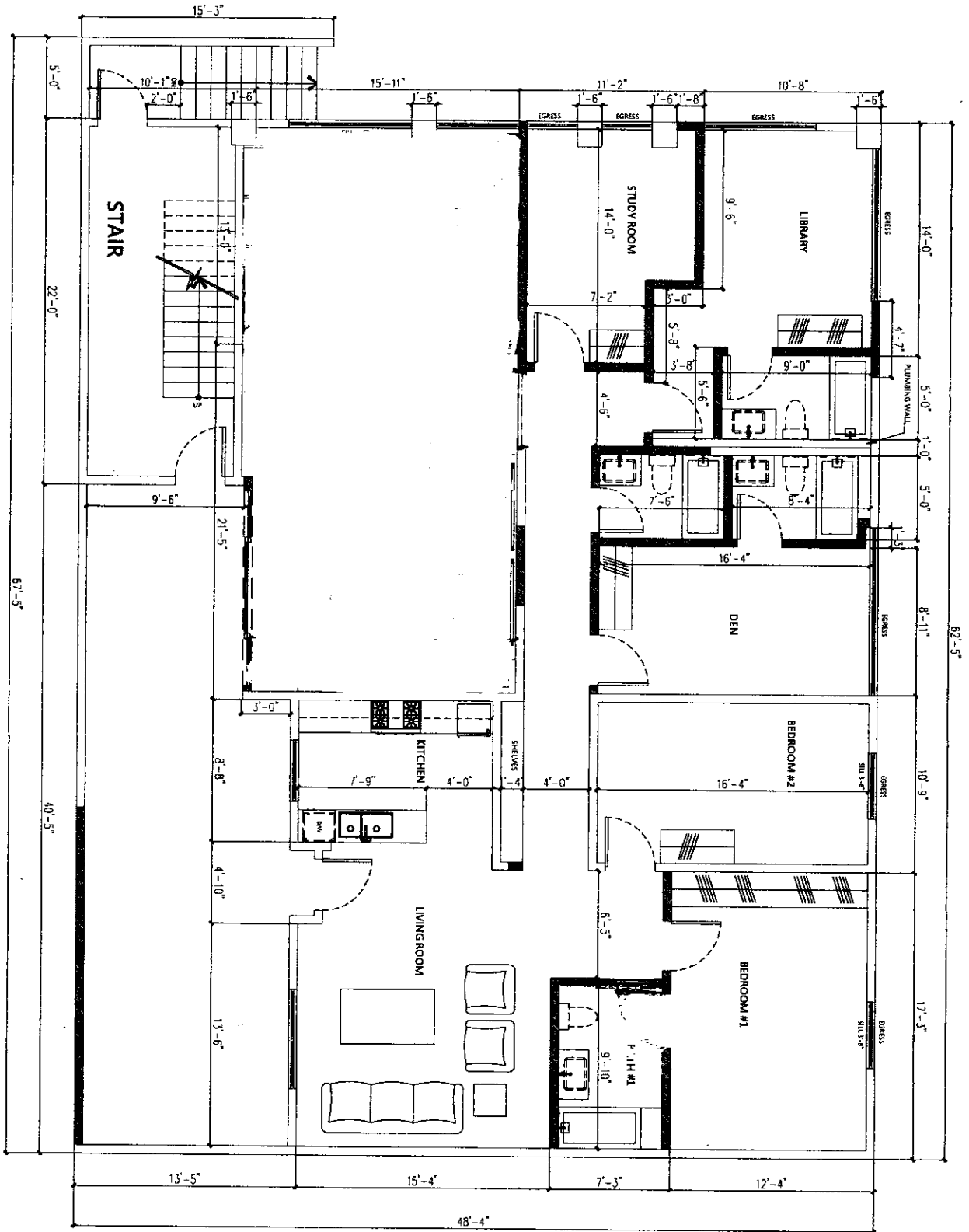
UNIT G-2 FLOOR PLAN
